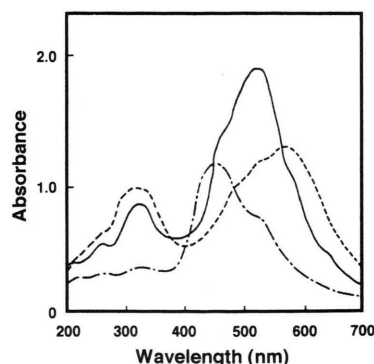
Fig. 5. Chromatoscanning traces of red, yellow and blue pigments separated by Sephadex LH-20 column. —: Red component (kinobeaon A); - - -: yellow component; ·····: blue component.
